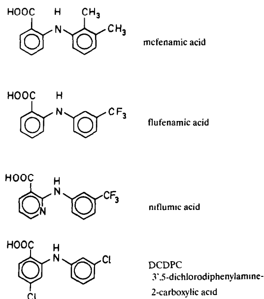
Fig. 1. Structural formula of blockers of the \text{Ca}^{2+} -activated non-selective cation channel.
